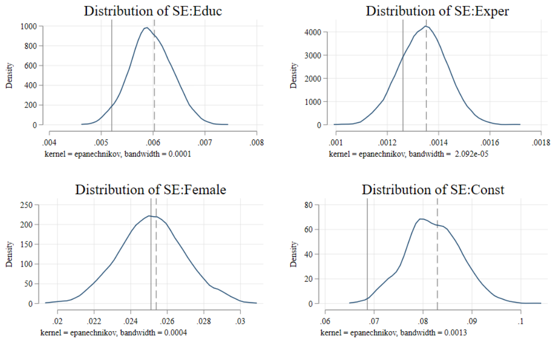
Figure 1: Standard Errors
